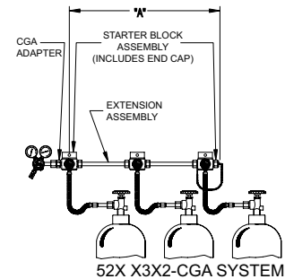
Regulator System
