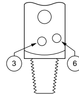
CGA 920 Pin-Indexed Yoke, Pins 3-6
