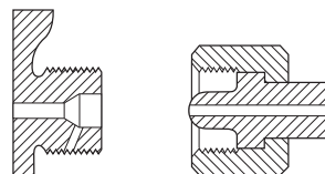
CGA 326 .825-14NGO-RH-EXT (Small Round Nipple)
