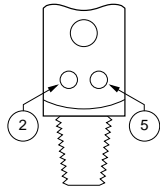
CGA 870 Pin-Indexed Yoke, Pins 2-5
