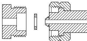
CGA 678 1.030-14NGO-LH-EXT (Recessed Washer)
