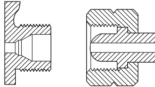
CGA 555 .903-14NGO-LH-EXT
