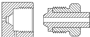
CGA 680 1.045-14NGO-RH-INT
