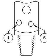
CGA 950 Pin-Indexed Yoke, Pins 1-5
