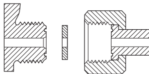
CGA 320 .825-14NGO-RH-EXT (Flat Nipple)
