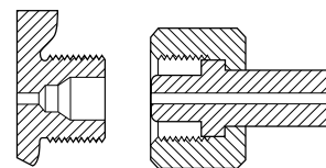
CGA 701 1.103-14NGO-RH-EXT
