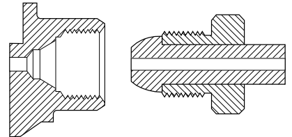
CGA 580 .965-14NGO-RH-INT
