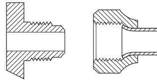
CGA 295 .750-16UNF-2A-RH-EXT (1/2" SAE Flare)
