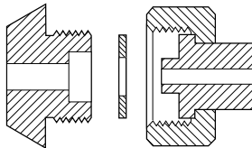
CGA 660 1.030-14NGO-RH-EXT (Face Washer)
