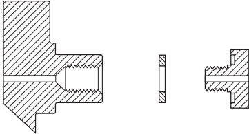
CGA 110 .3125-32UNEF-2B-RH-INT
