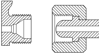
CGA 540 .903-14NGO-RH-EXT
