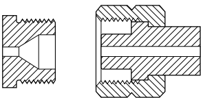
CGA 677 1.030-14NGO-LH-EXT (Round Nipple)
