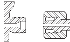
CGA 280 .745-14NGO-RH-EXT
