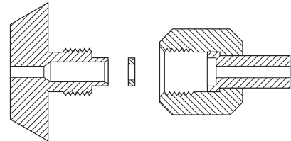
CGA 280 .745-14NGO-RH-EXT
