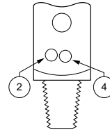
CGA 890 Pin-Indexed Yoke, Pins 2-4
