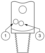
CGA 900 Pin-Indexed Yoke, Pins 1-3
