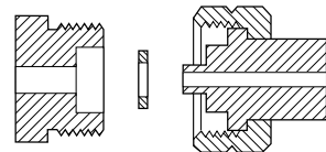
CGA 679 1.030-14NGO-LH-EXT (Tipped Nipple)
