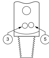
CGA 910 Pin-Indexed Yoke, Pins 3-5
