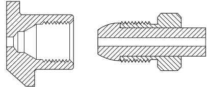
CGA 296 .803-14UNS-2B-RH-INT
