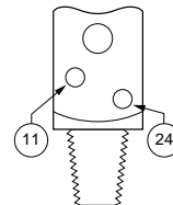
CGA 973 Pin-Indexed Yoke, Pins 11-24
