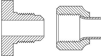
CGA 440 .875-14UNF-2A-RH-EXT (5/8" SAE Flare)
