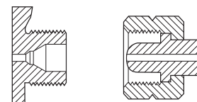
CGA 350 .825-14NGO-LH-EXT (Round Nipple)
