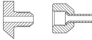
CGA 240 .375-18NGT-RH-INT
