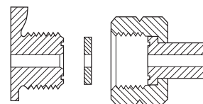
CGA 330 .825-14NGO-LH-EXT (Flat Nipple)
