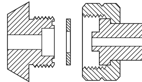
CGA 670 1.030-14NGO-LH-EXT (Face Washer)
