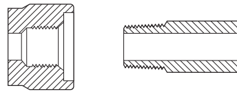
CGA 240 .375-18NGT-RH-INT
