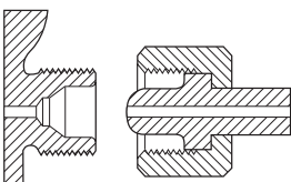
CGA 346 .825-14NGO-RH-EXT (Large Round Nipple)
