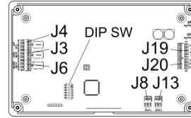
Figure 11 for Circuit Board Style A ("CV1")
