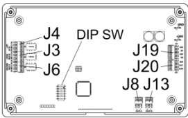
Figure 15 for Circuit Board Style A ("CV1")
