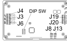
Figures 16 & 17 for Circuit Board Style A ("CV1")
