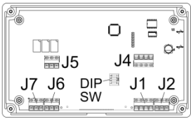
Figures 16 & 17 for Circuit Board Style B ("CE")
