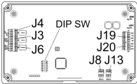
Figure 10 for Circuit Board Style A ("CV1")
