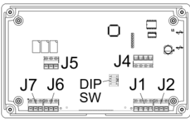
Figure 12 for Circuit Board Style B ("CE")
