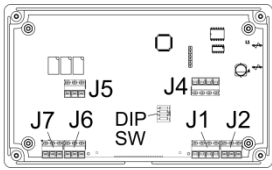
Figure 18 for Circuit Board Style B ("CE")
