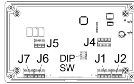
Figure 6 for Circuit Board Style B ("CE")
