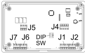
Figure 14 for Circuit Board Style B ("CE")
