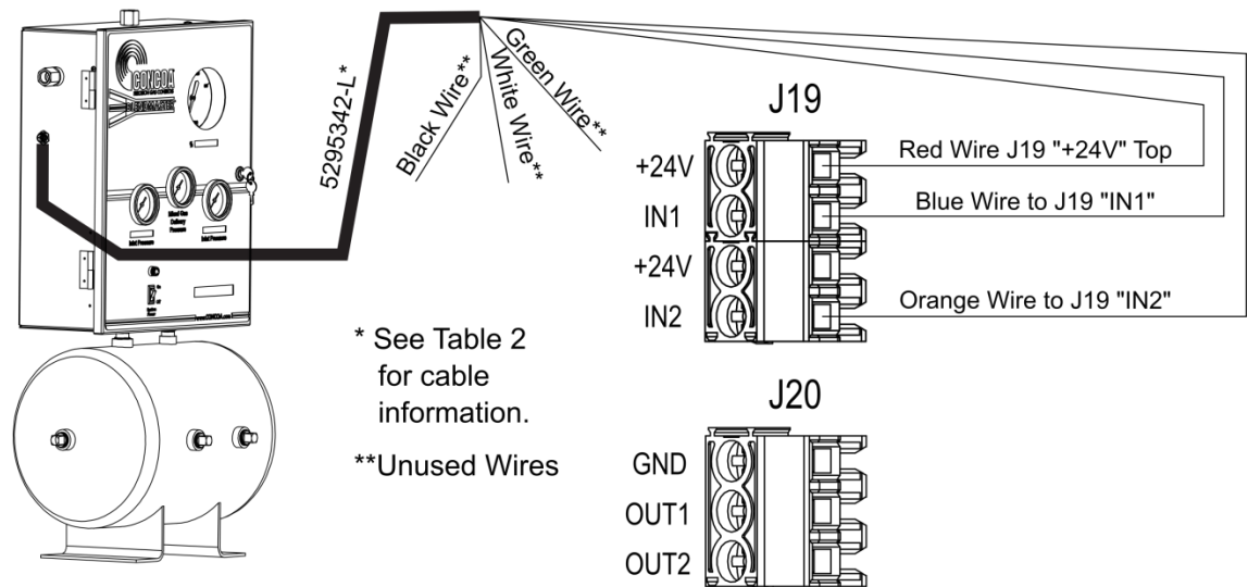
Figure 18 for Circuit Board Style B ("CE")
