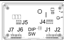
Figure 10 for Circuit Board Style B ("CE")
