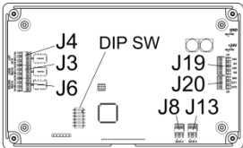
Figure 13 for Circuit Board Style A ("CV1")
