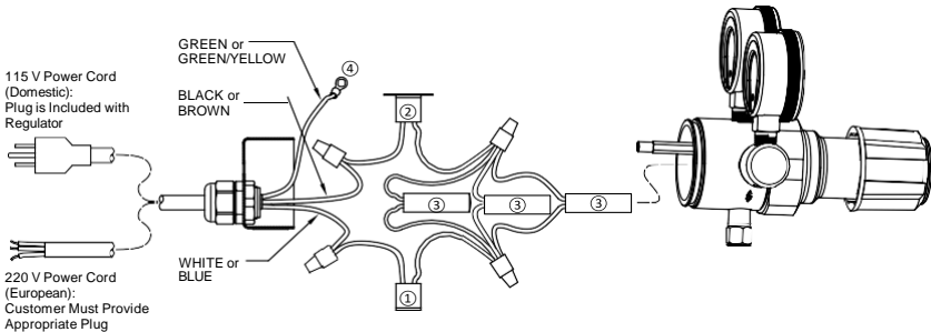
WIRING DIAGRAM
