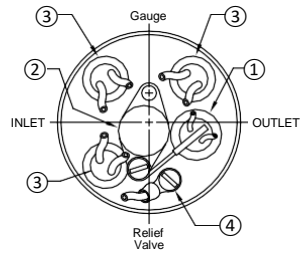
VIEW OF HEATERS & THERMOSTATS INSTALLED IN BACK OF REGULATOR
