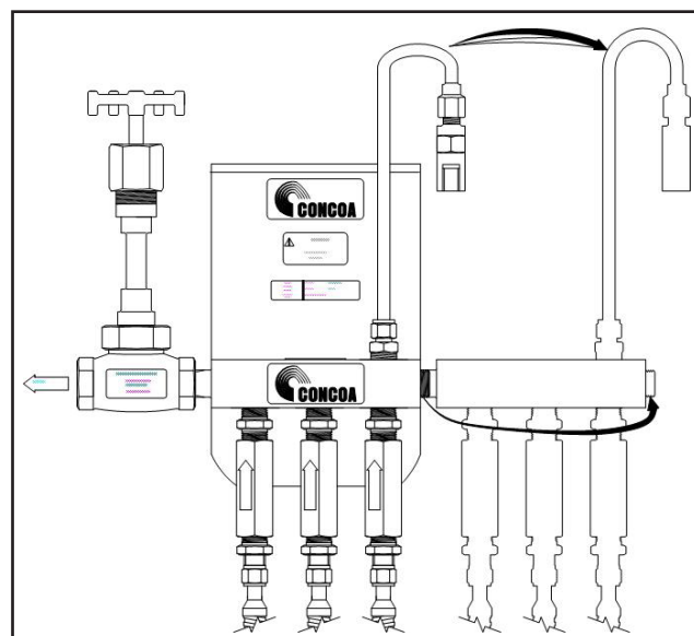
Figure 4 - Manifold extension assembly
